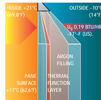
UNILUX WARM GLASS 1.1 (U g 0,19 BTU/HR-FT 2 -F (US)). (CROSS SECTION)
